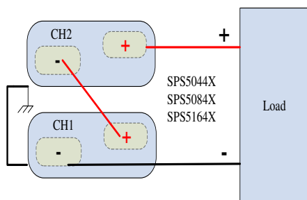
Dual-channel Series Connection
