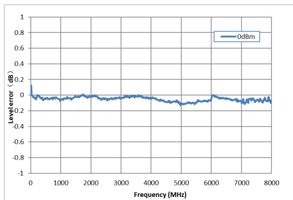
Measured level error versus frequency, Level = 0 dBm
