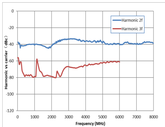
Measured harmonics versus carrier frequency at level \leq +13 \text{ dBm}
