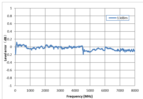
Measured level error versus frequency, Level = +13 dBm
